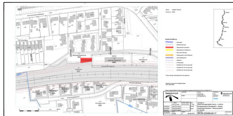
Skørping Station (autotransformer)
